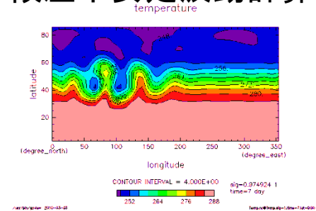
Temperature at lowest level at 7th day, T21L20
