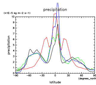
Figure 100: Rain at Apr. by DCPAM (red), NCEP (green), ECMWF (blue), and GPCP (black)
