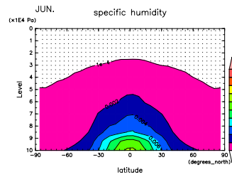
Figure 412: q at Jun. by DCPAM
