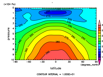
Figure 371: T at Apr. by NCEP
