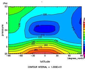
Figure 686: T at Jan. by NCEP
