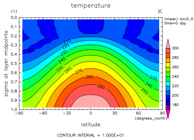
Figure 4: Zonal mean temperature by DCPAM
