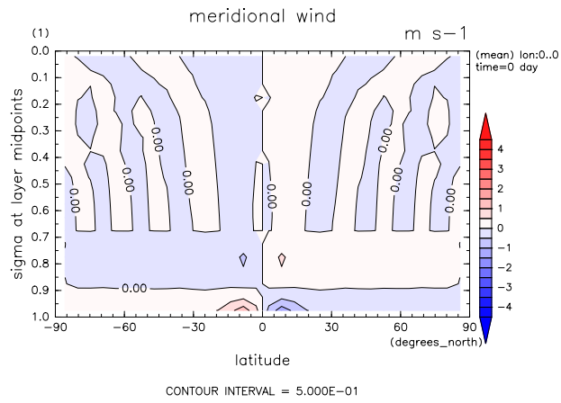
Figure 2: Zonal mean meridional wind by DCPAM
