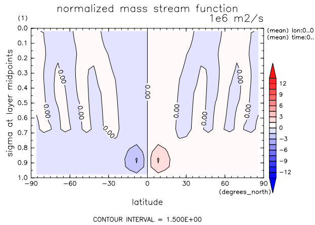
Figure 3: Normalized mass stream function by DCPAM
