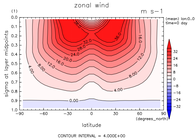
Figure 1: Zonal mean zonal wind by DCPAM
