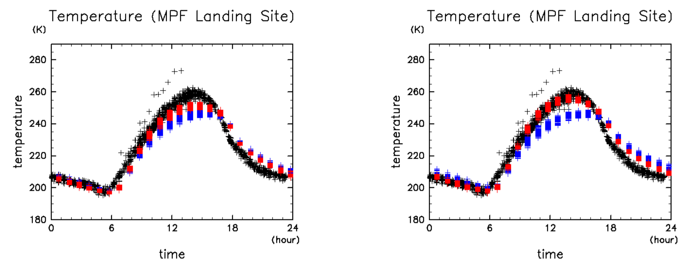
Figure 3: Diurnal variation of ground and atmospheric temperatures: black mark indicates MPF observation at 1.5 m height: (left panel) Blue mark indicates lowest level (about 3 m height) model temperature and red mark indicates estimated atmospheric temperature at 1.5 m height (right panel) Same as left panel but 2nd level (about 12.5 m height) model temperature (blue mark) is used for estimation of temperature at 1.5 m height.
