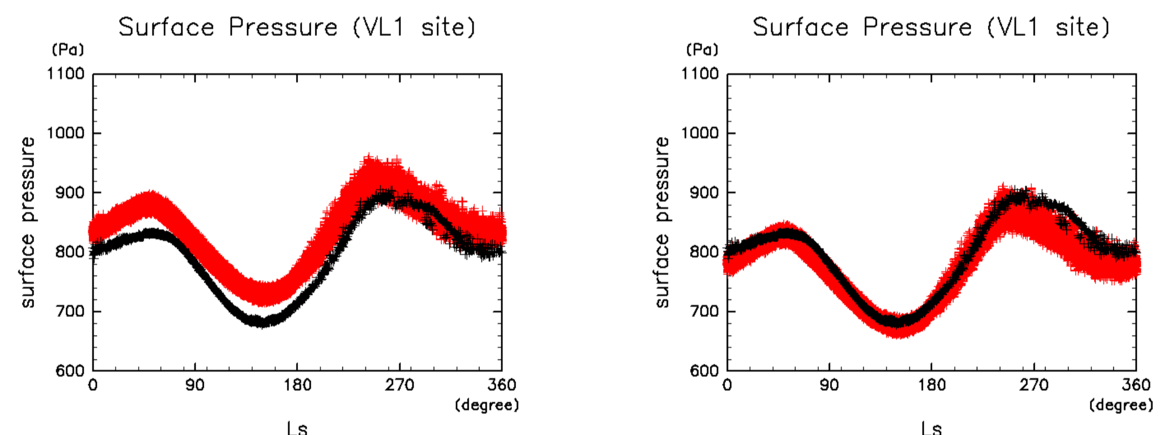
Figure 4: Seasonal variation of surface pressure at Viking Lander 1 site: black mark indicates VL1 results and red mark indicates model surface pressure: (left panel) before calibration and (right panel) after calibration.
