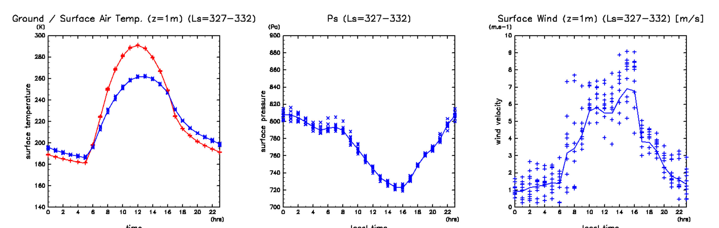
Figure 6: Diurnal variation of ground and 1 m height atmospheric temperatures (left panel), surface pressure (middle panel), and surface wind velocity (right panel) at Juventae Chasma from Ls=327° to 332°. Solid line in each figure indicates mean value.
