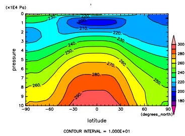
Figure 395: T at Dec. by NCEP
