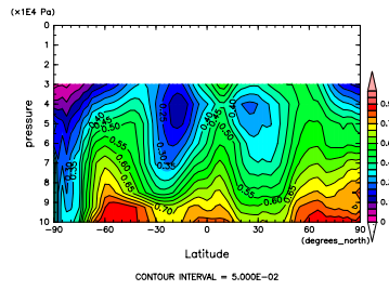
Figure 457: RH at Sep. by DCPAM
