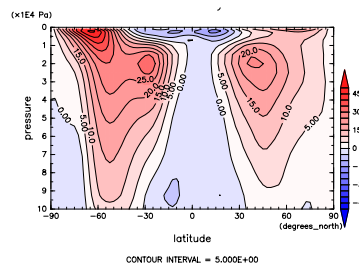
Figure 245: U at Oct. by NCEP
