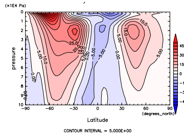
Figure 241: U at Sep. by DCPAM
