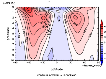
Figure 244: U at Oct. by DCPAM
