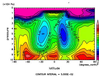
Figure 467: RH at Dec. by NCEP
