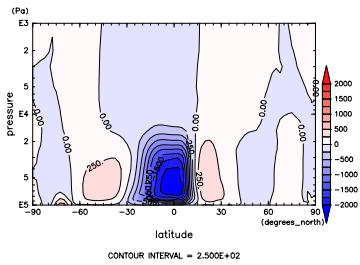
Figure 674: MSF at Sep. by NCEP
