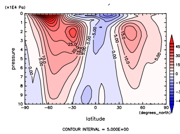
Figure 242: U at Sep. by NCEP
