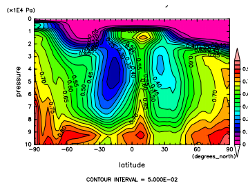
Figure 458: RH at Sep. by NCEP
