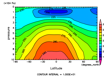
Figure 364: T at Feb. by DCPAM
