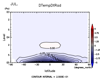
Figure 859: (\partial T / \partial t)_{SW+LW} at Jul. by DCPAM
