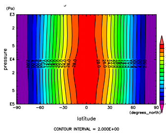
Figure 608: ANG MOM at Nov. by NCEP
