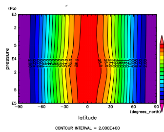
Figure 611: ANG MOM at Dec. by NCEP
