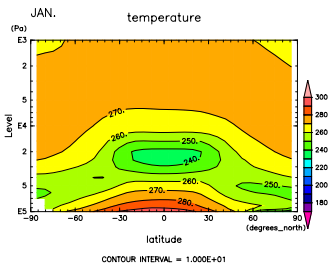
Figure 685: T at Jan. by DCPAM
