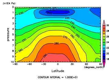
Figure 361: T at Jan. by DCPAM
