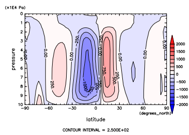
Figure 29: Annual mean MSF by NCEP
