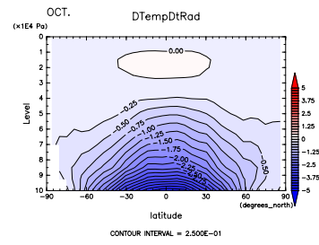
Figure 538: (\partial T / \partial t)_{SW+LW} at Oct. by DCPAM
