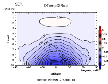
Figure 537: (\partial T / \partial t)_{SW+LW} at Sep. by DCPAM
