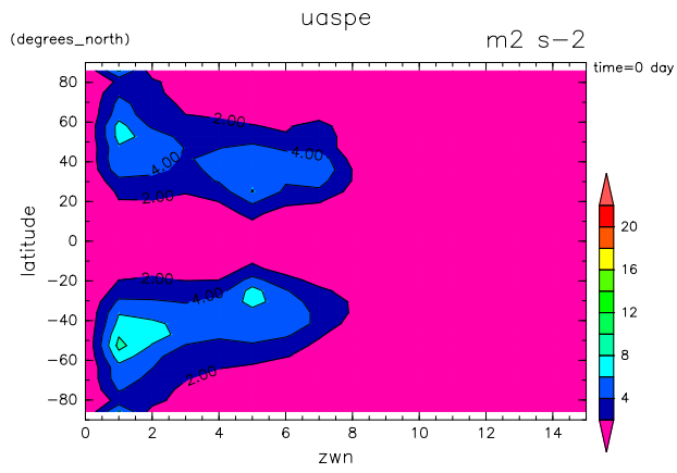
Figure 5: Spectrum of zonal wind by DCPAM
