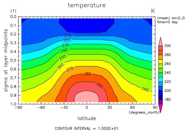
Figure 2: Zonal mean temperature by DCPAM
