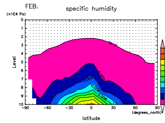
Figure 400: q at Feb. by DCPAM
