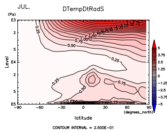
Figure 835: (\partial T/\partial t)_{SW} at Jul. by DCPAM
