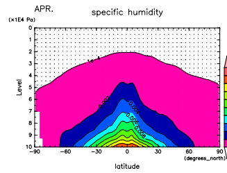
Figure 406: q at Apr. by DCPAM
