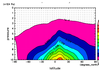
Figure 419: q at Aug. by NCEP
