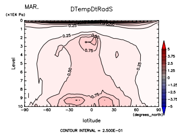
Figure 507: (\partial T/\partial t)_{sw} at Mar. by DCPAM
