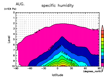
Figure 418: q at Aug. by DCPAM
