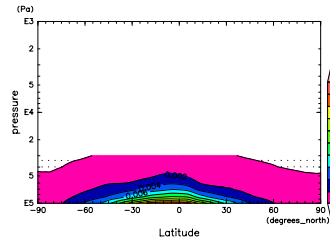
Figure 724: q at Feb. by DCPAM
