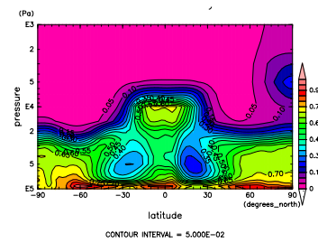
Figure 791: RH at Dec. by NCEP
