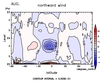
Figure 634: V at Aug. by DCPAM
