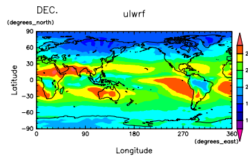
Figure 154: OLR at Dec. by DCPAM
