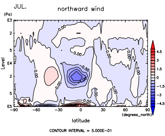
Figure 631: V at Jul. by DCPAM
