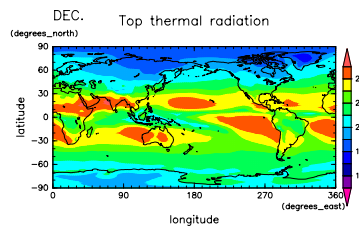
Figure 155: OLR at Dec. by NCEP
