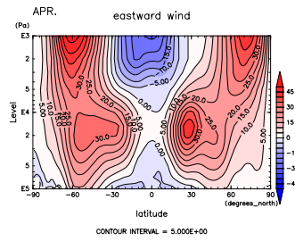
Figure 550: U at Apr. by DCPAM
