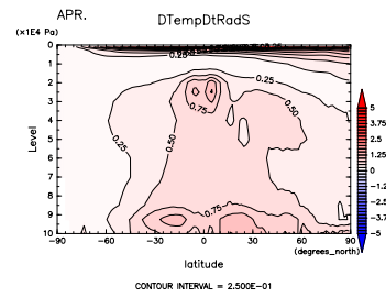
Figure 508: (\partial T/\partial t)_{sw} at Apr. by DCPAM
