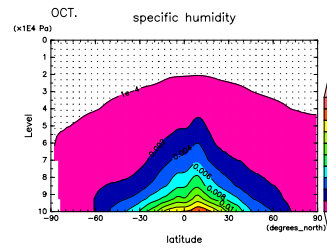
Figure 424: q at Oct. by DCPAM
