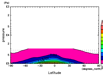
Figure 721: q at Jan. by DCPAM
