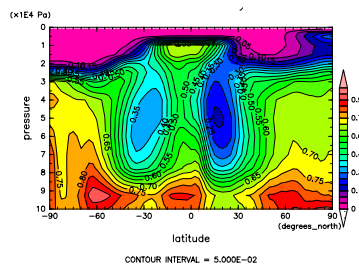
Figure 434: RH at Jan. by NCEP
