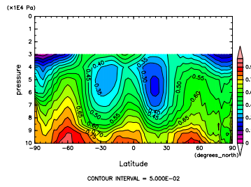
Figure 433: RH at Jan. by DCPAM
