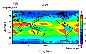
Figure 121: OLR at Jan. by DCPAM Figure 124: OLR at Feb. by DCPAM
