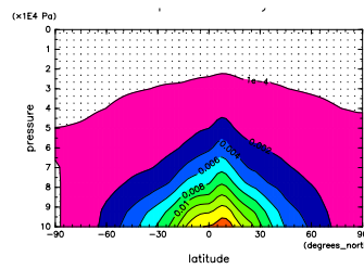
Figure 425: q at Oct. by NCEP
