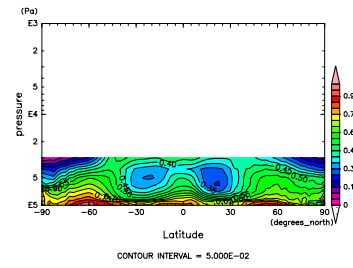
Figure 790: RH at Dec. by DCPAM
