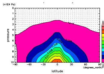
Figure 407: q at Apr. by NCEP
