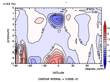
Figure 314: V at Sep. by NCEP
