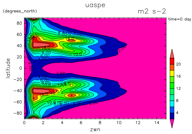
Figure 8: Spectrum of zonal wind by DCPAM
