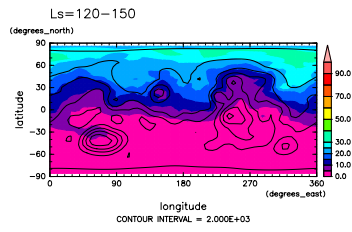
Figure 369: Prec. water at 14 LST and Ls=90°-120° by DCPAM
