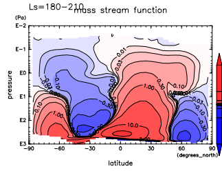
Figure 106: MSF at L_S=180^\circ-210^\circ by DCPAM
