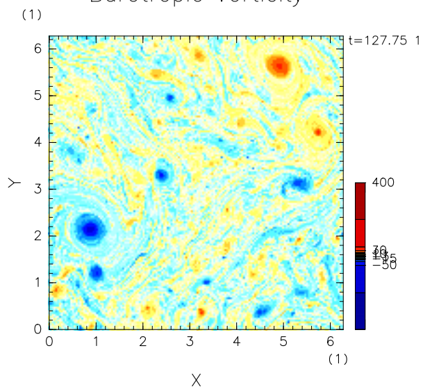
Barotropic Vorticity
