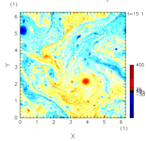
Baroclinic Vorticity
