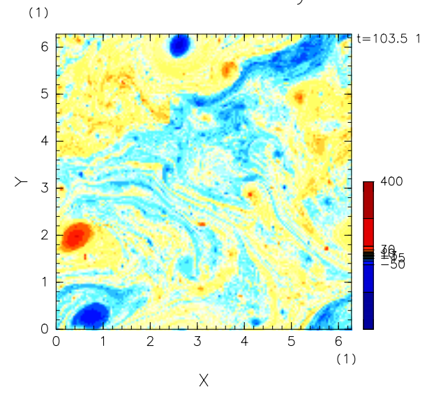
Baroclinic Vorticity
