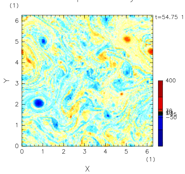
Barotropic Vorticity
