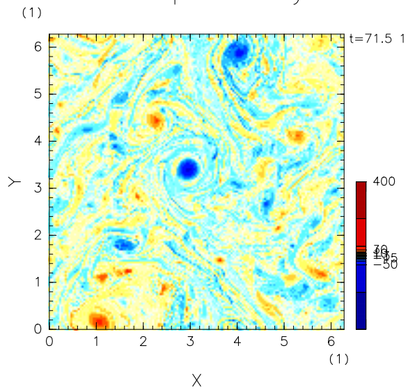
Barotropic Vorticity
