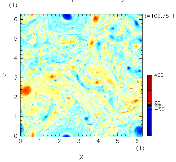
Barotropic Vorticity
