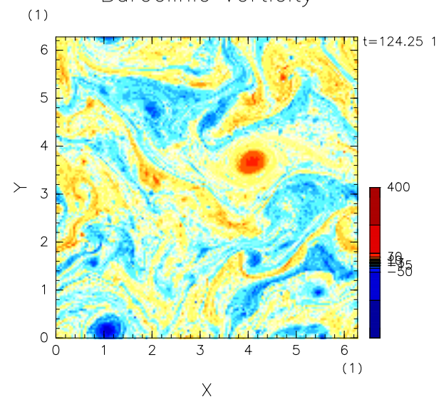
Baroclinic Vorticity
