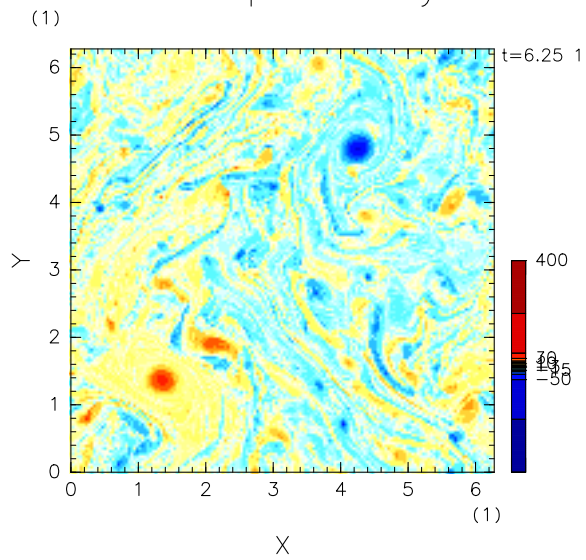
Barotropic Vorticity
