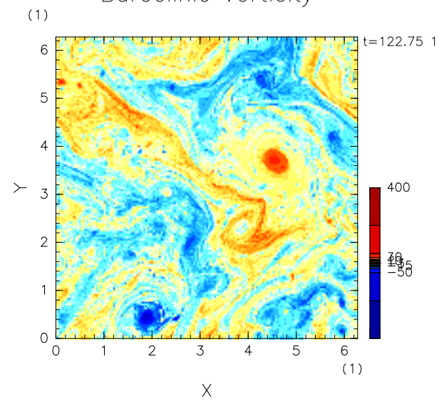
Baroclinic Vorticity
