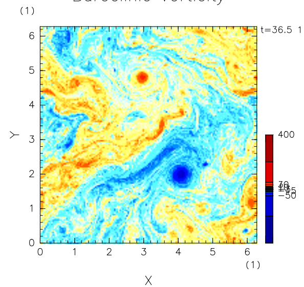
Baroclinic Vorticity
