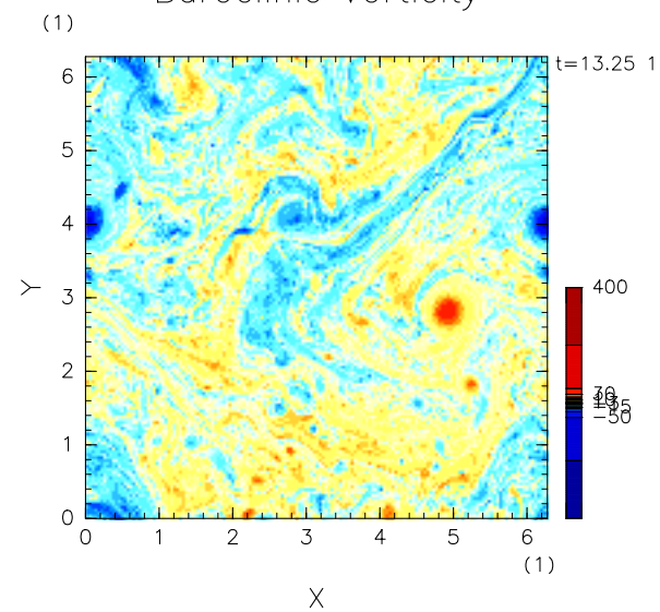
Baroclinic Vorticity
