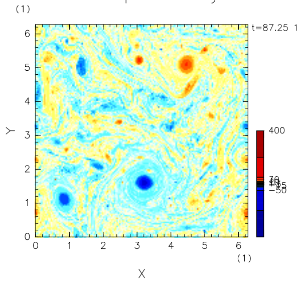
Barotropic Vorticity
