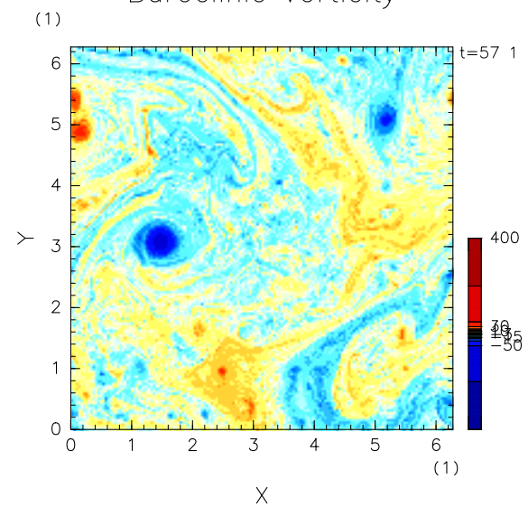
Baroclinic Vorticity
