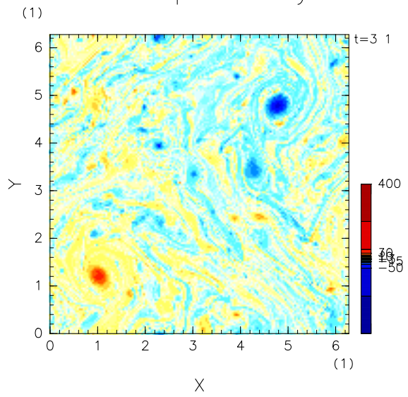
Barotropic Vorticity
