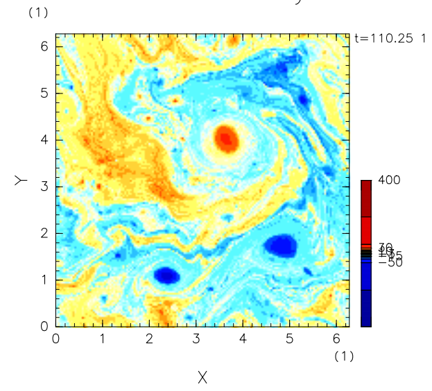
Baroclinic Vorticity
