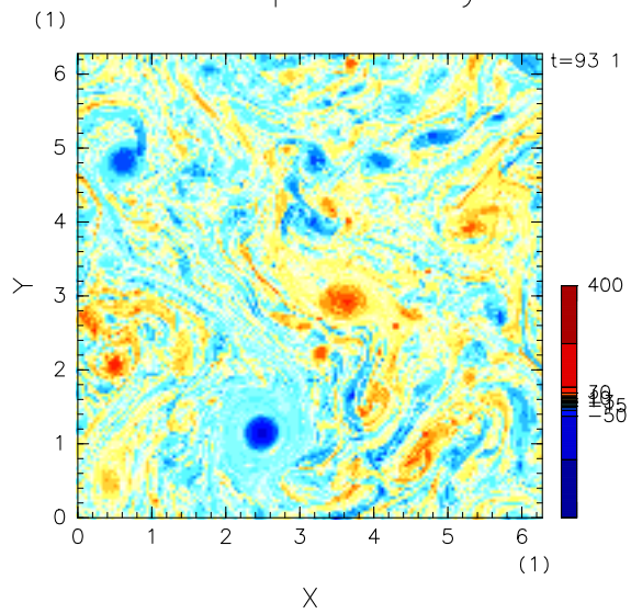
Barotropic Vorticity
