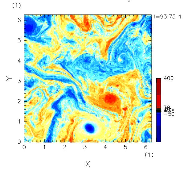
Baroclinic Vorticity
