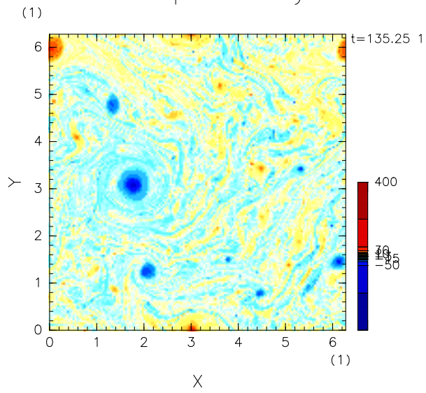
Barotropic Vorticity
