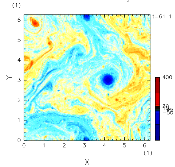
Baroclinic Vorticity
