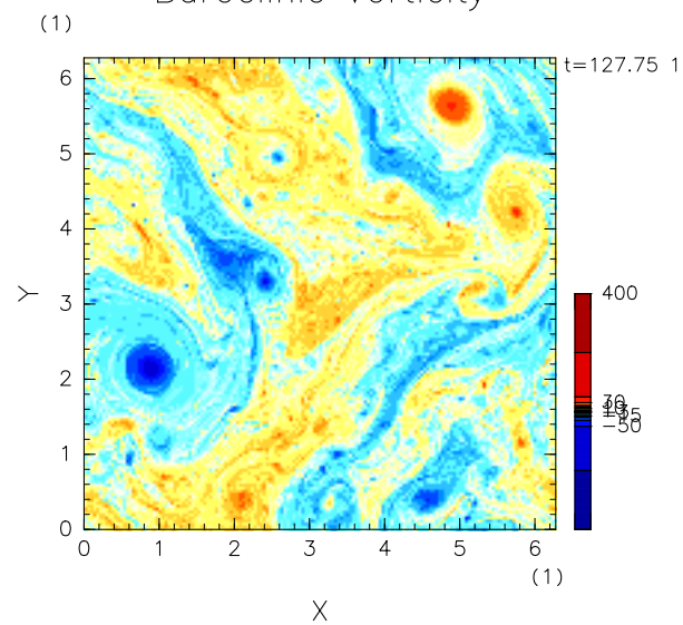
Baroclinic Vorticity
