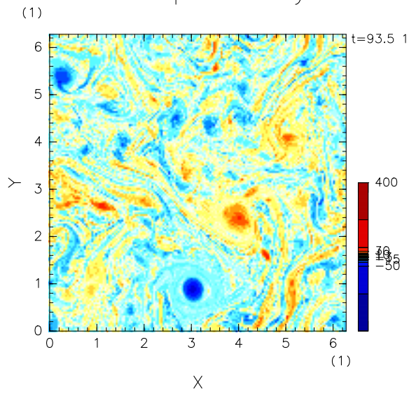
Barotropic Vorticity
