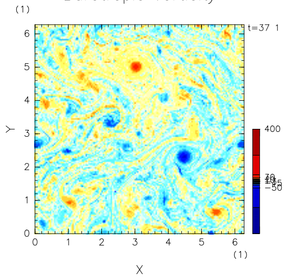
Barotropic Vorticity
