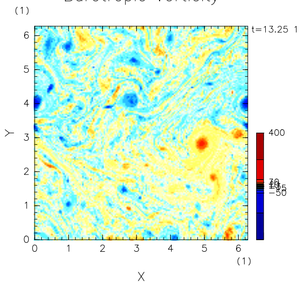
Barotropic Vorticity
