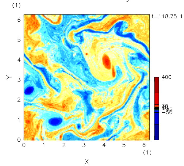
Baroclinic Vorticity
