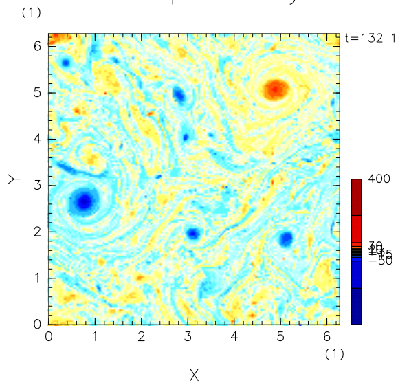
Barotropic Vorticity
