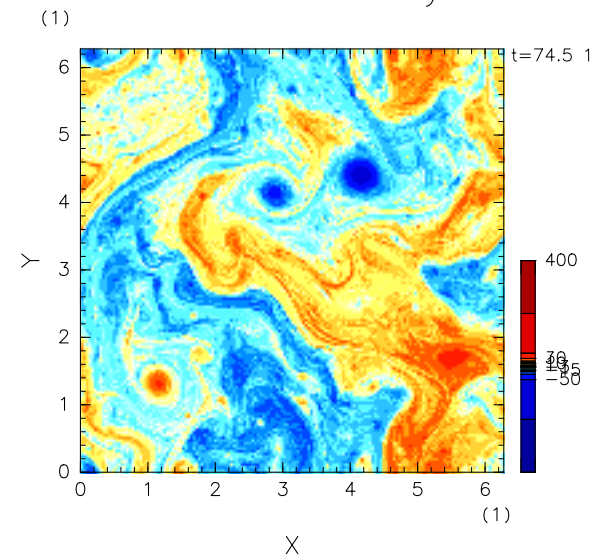
Baroclinic Vorticity
