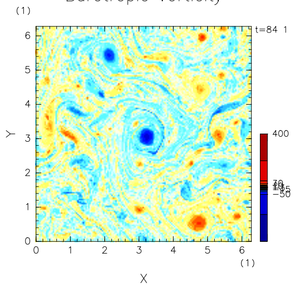
Barotropic Vorticity
