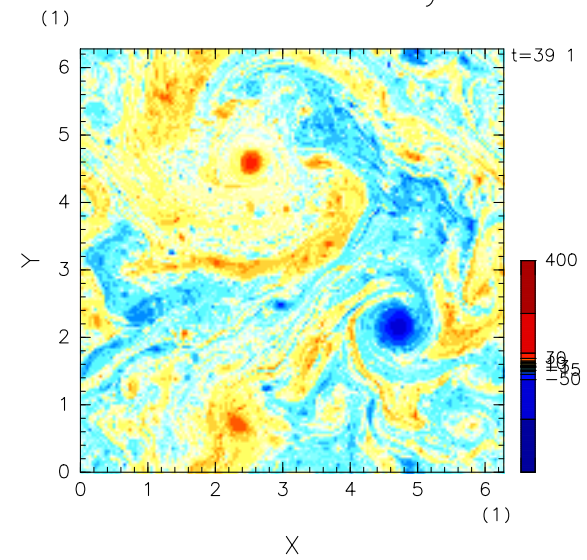
Baroclinic Vorticity
