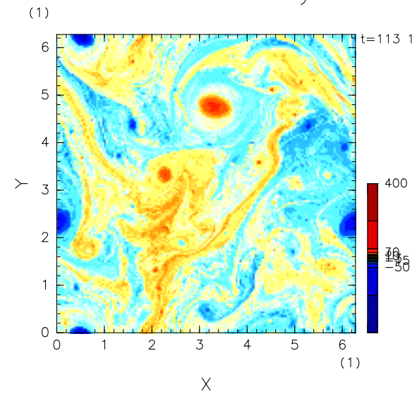
Baroclinic Vorticity
