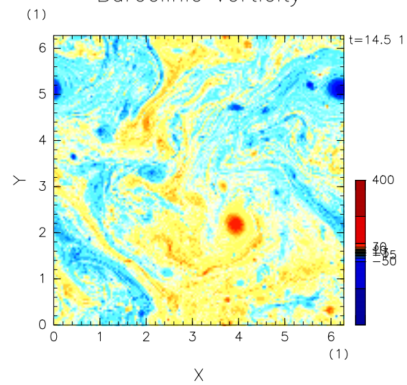
Baroclinic Vorticity
