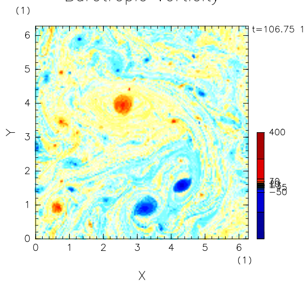
Barotropic Vorticity
