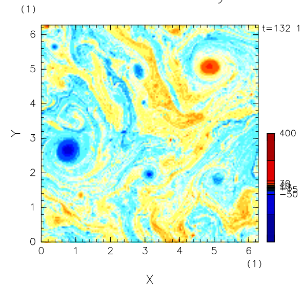
Baroclinic Vorticity
