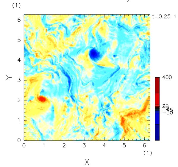
Baroclinic Vorticity
