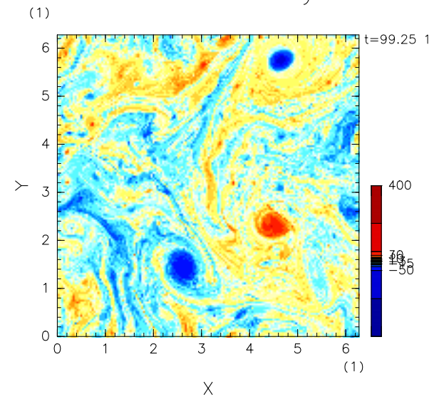
Baroclinic Vorticity
