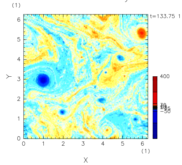
Baroclinic Vorticity
