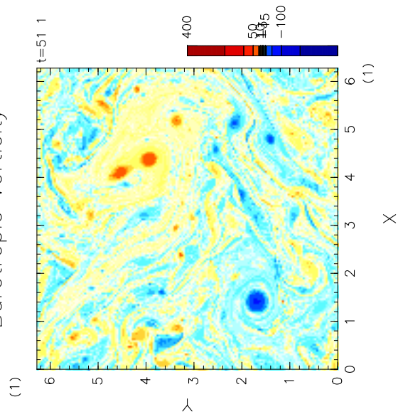
Barotropic Vorticity
